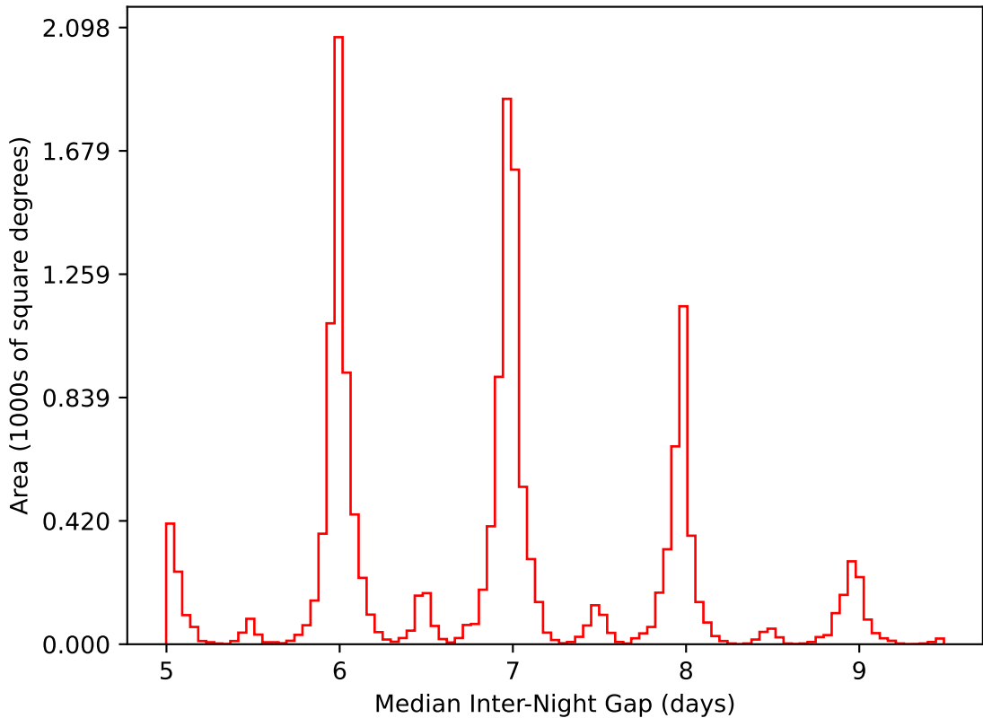
too_elab_r16_d2_giz_v3.4_10yrs WFD i band: Median Inter-Night Gap
