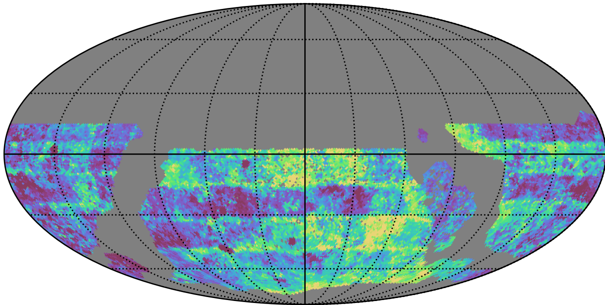
too_elab_r16_d2_giz_v3.4_10yrs WFD g band: Median Inter-Night Gap
