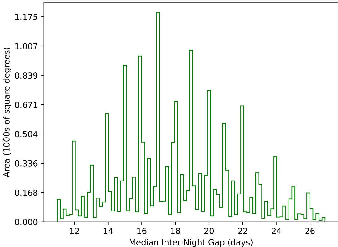
too_elab_r16_d2_giz_v3.4_10yrs WFD g band: Median Inter-Night Gap
