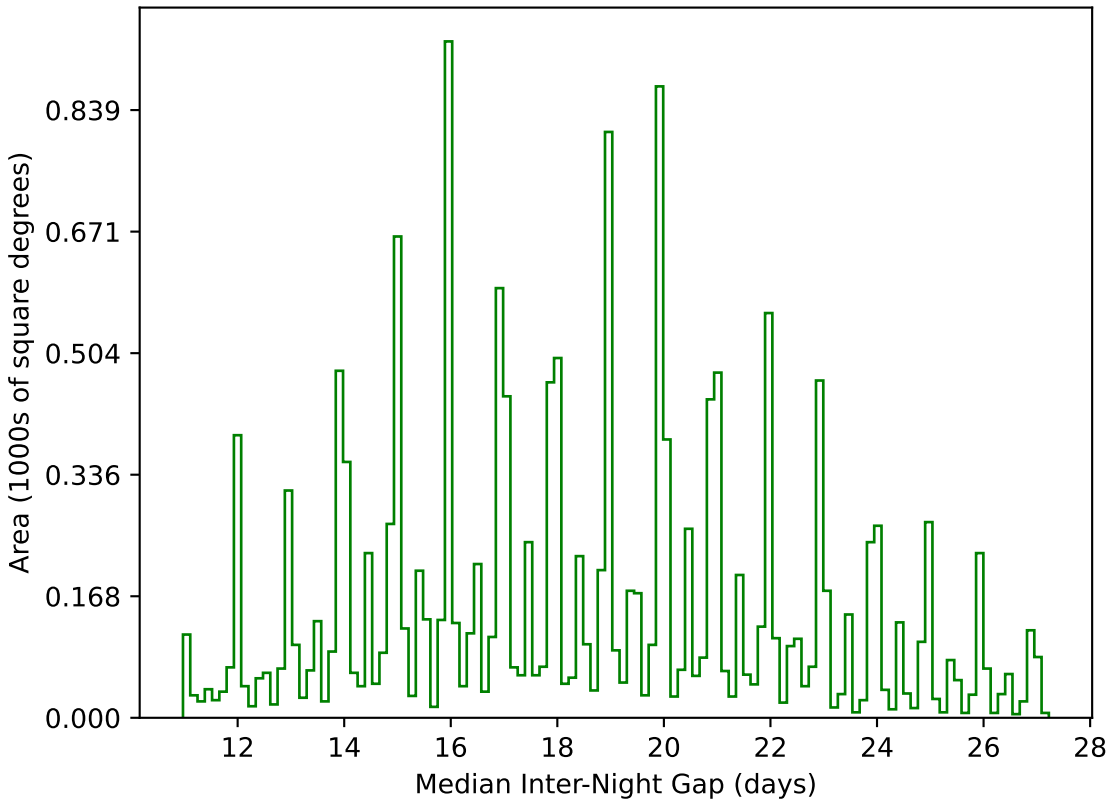
too_elab_r16_d2_giz_v3.4_10yrs WFD g band: Median Inter-Night Gap
