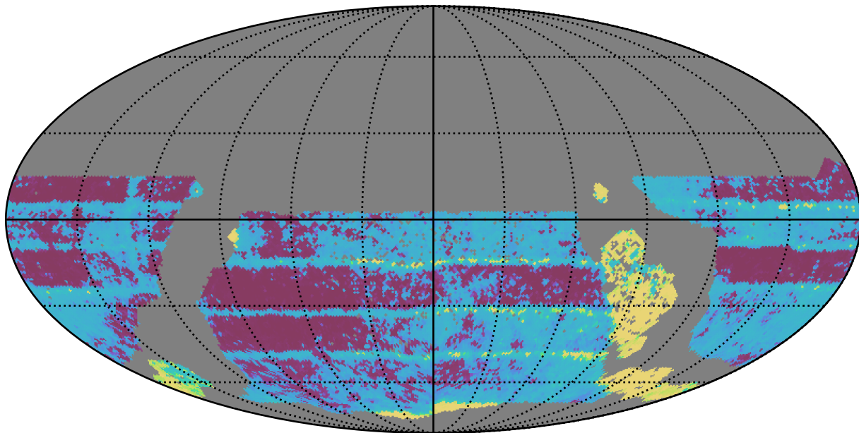
too_elab_r16_d2_giz_v3.4_10yrs WFD all bands: Median Inter-Night Gap
