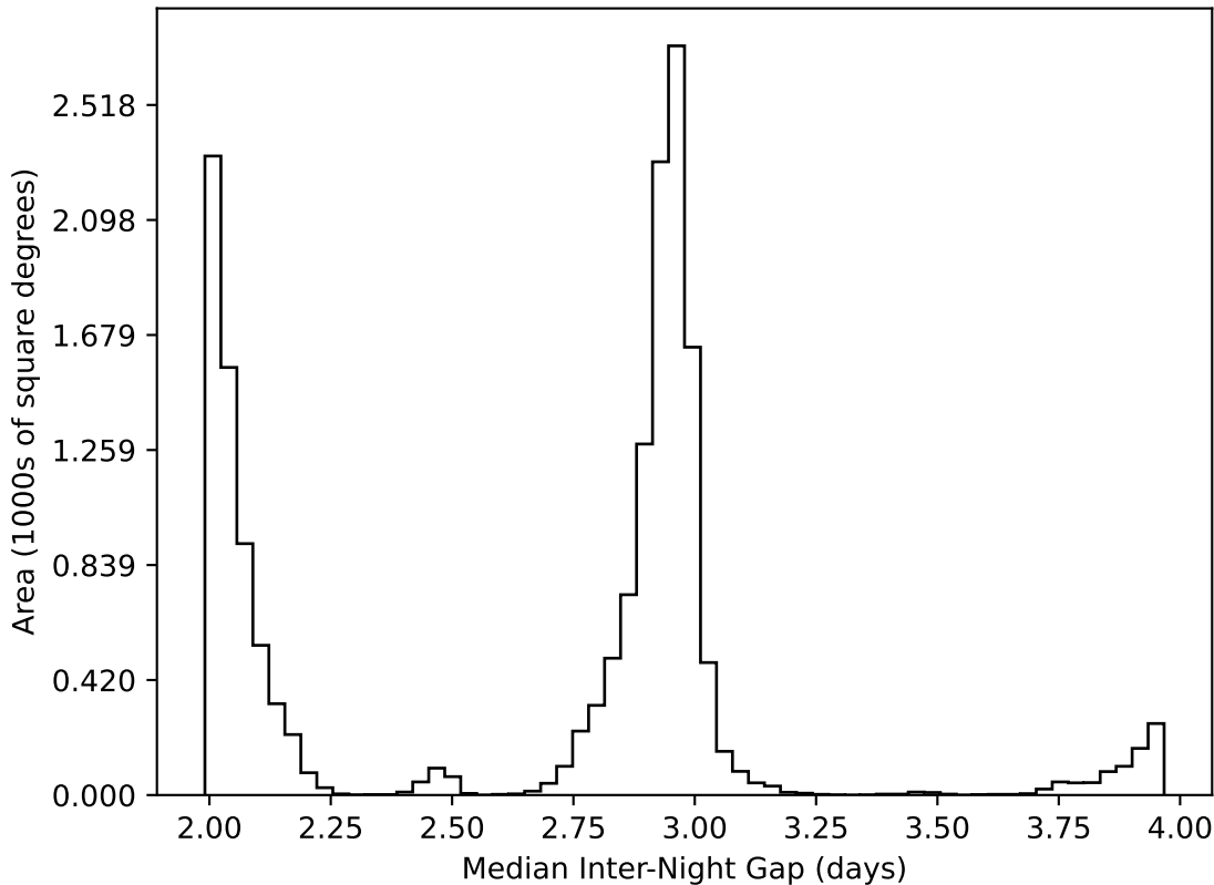
too_elab_r16_d2_giz_v3.4_10yrs WFD all bands: Median Inter-Night Gap
