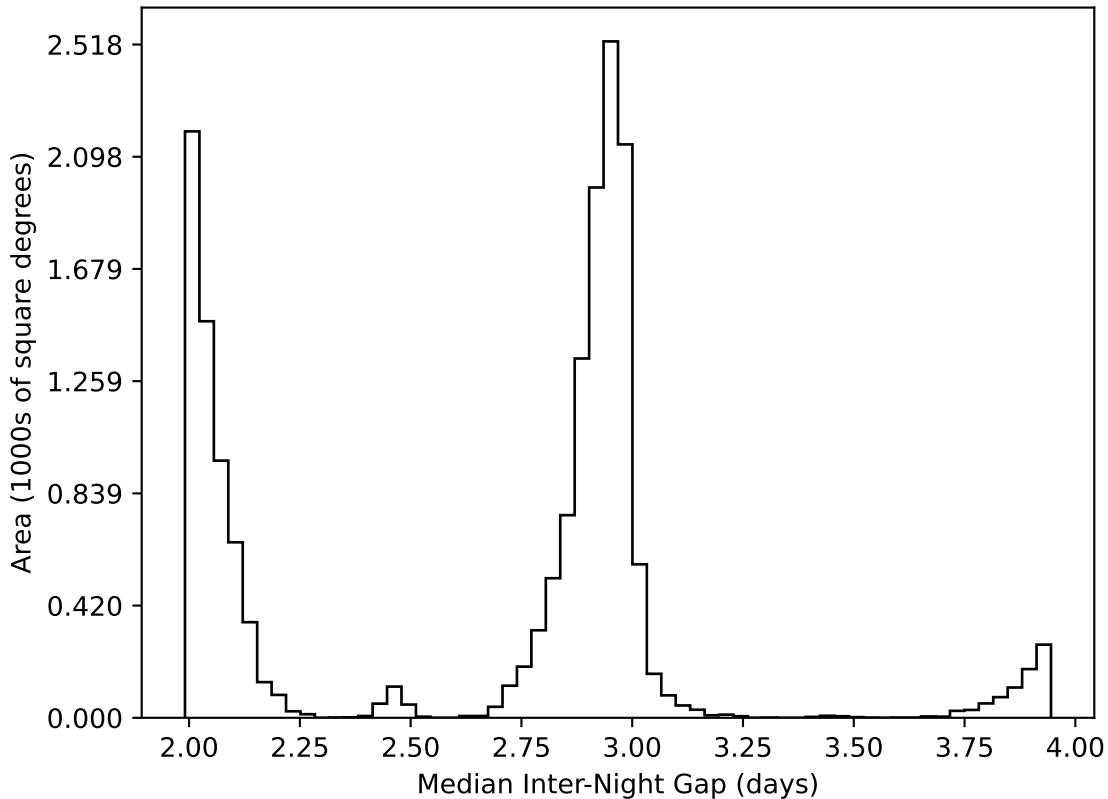
too_elab_r16_d2_giz_v3.4_10yrs WFD all bands: Median Inter-Night Gap
