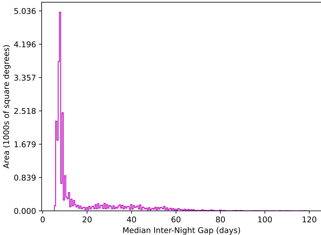
too_elab_r16_d2_giz_v3.4_10yrs All sky z band: Median Inter-Night Gap
