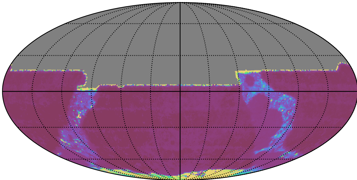
too_elab_r16_d2_giz_v3.4_10yrs All sky y band: Median Inter-Night Gap
