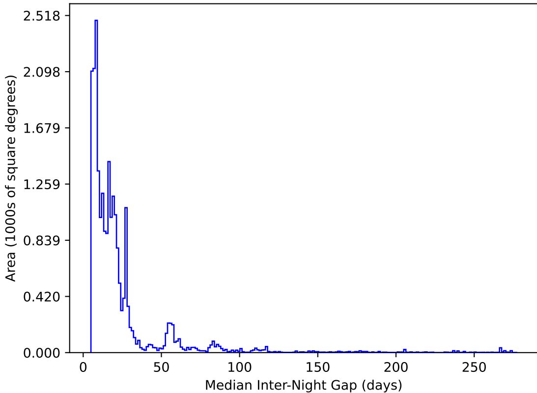
too_elab_r16_d2_giz_v3.4_10yrs All sky y band: Median Inter-Night Gap
