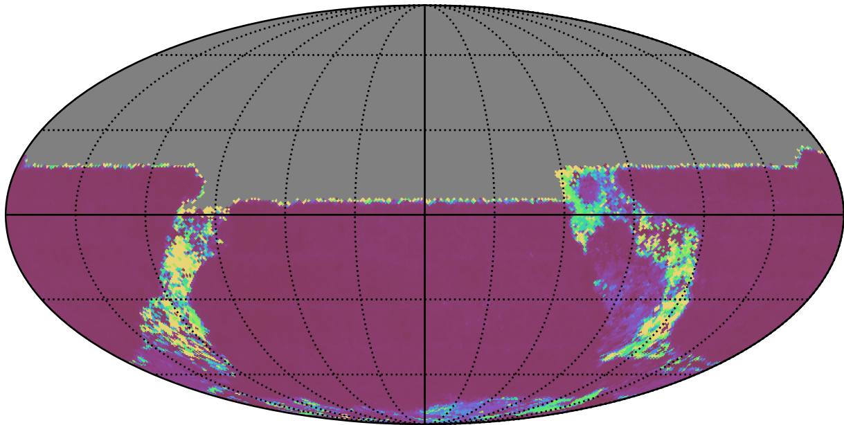
too_elab_r16_d2_giz_v3.4_10yrs All sky u band: Median Inter-Night Gap
