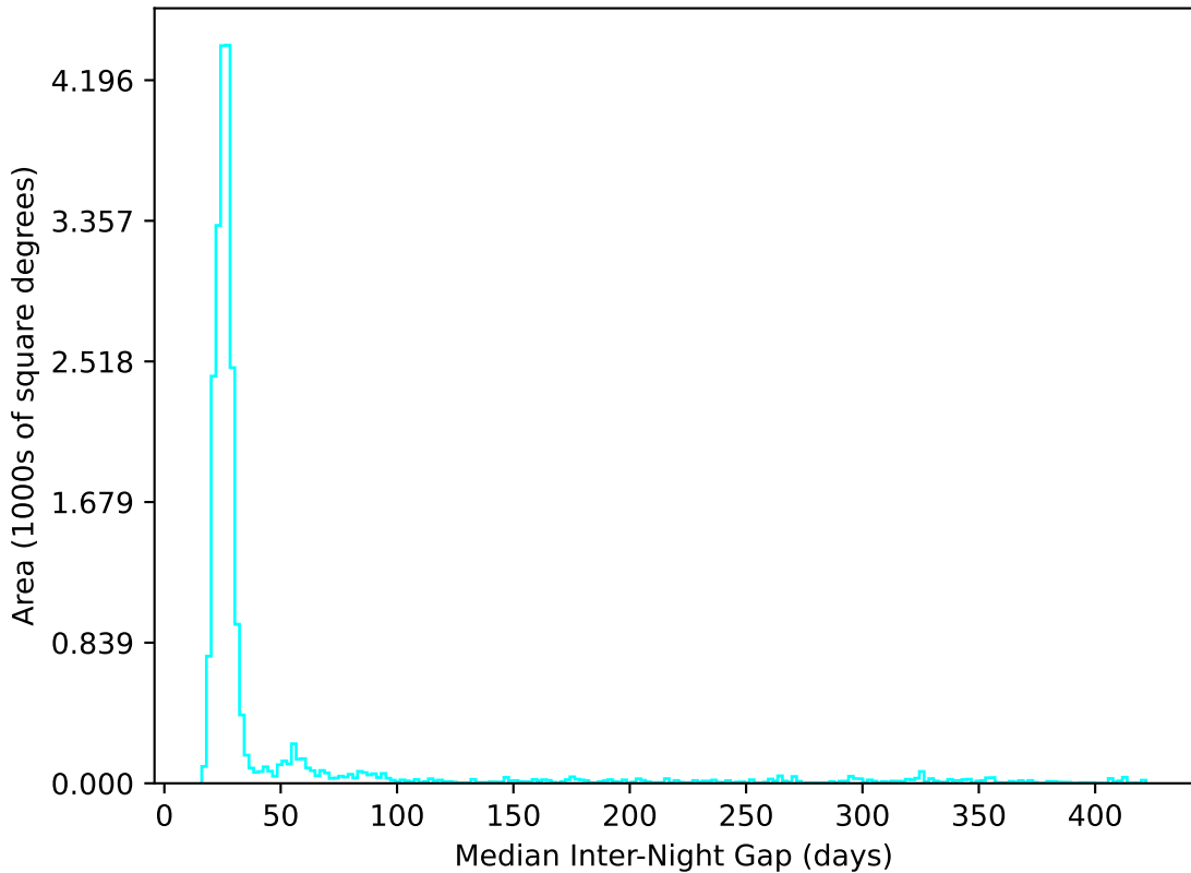
too_elab_r16_d2_giz_v3.4_10yrs All sky u band: Median Inter-Night Gap
