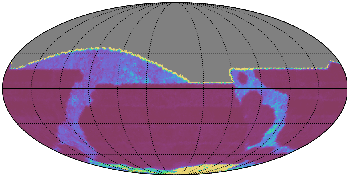
too_elab_r16_d2_giz_v3.4_10yrs All sky r band: Median Inter-Night Gap
