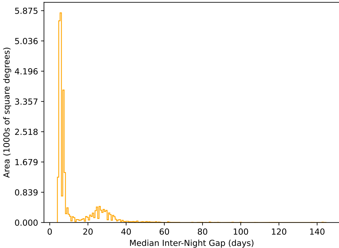
too_elab_r16_d2_giz_v3.4_10yrs All sky r band: Median Inter-Night Gap
