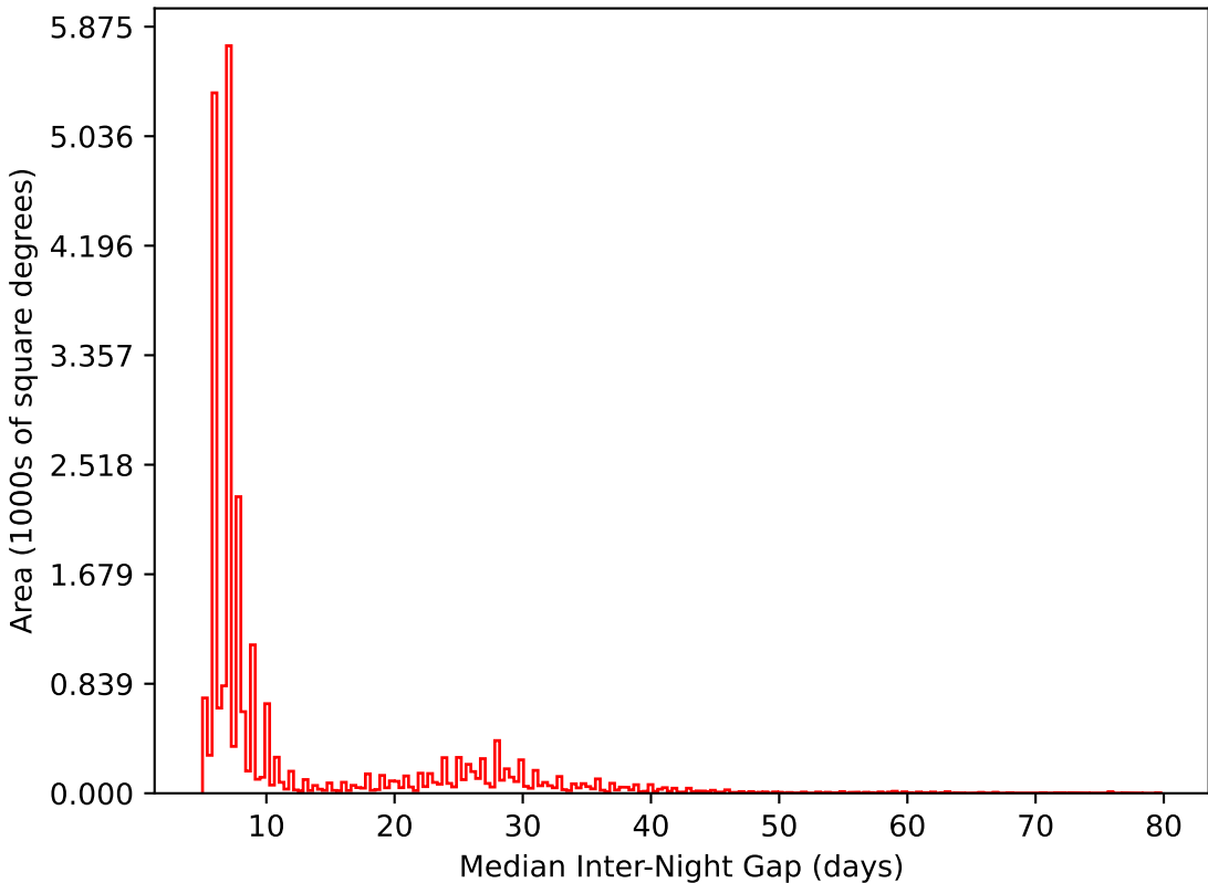
too_elab_r16_d2_giz_v3.4_10yrs All sky i band: Median Inter-Night Gap
