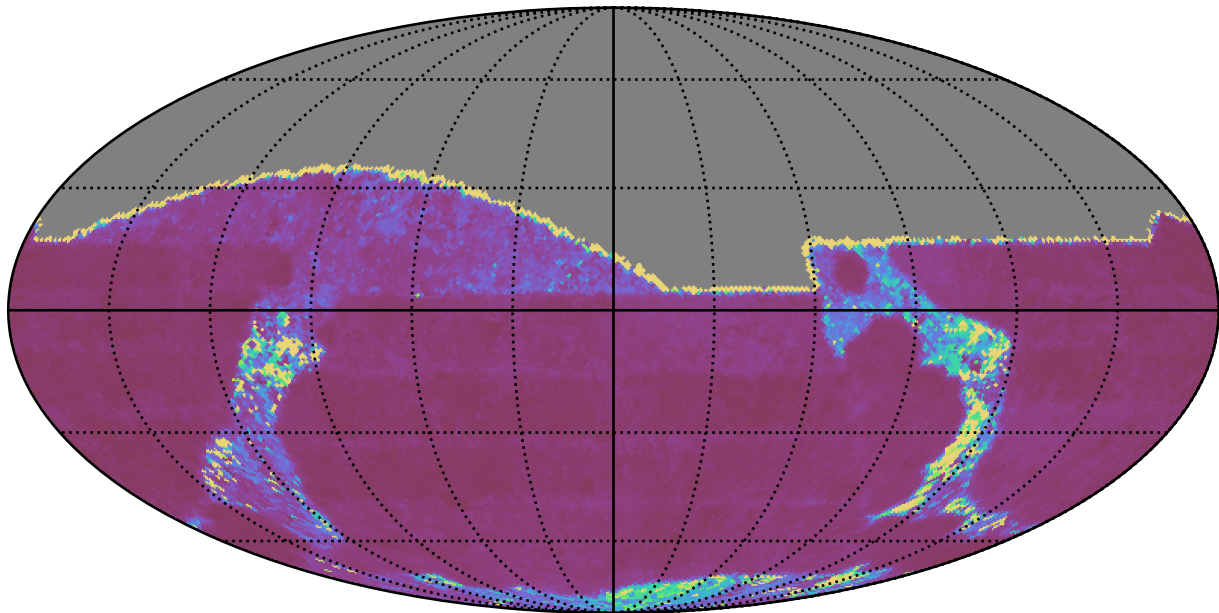
too_elab_r16_d2_giz_v3.4_10yrs All sky g band: Median Inter-Night Gap
