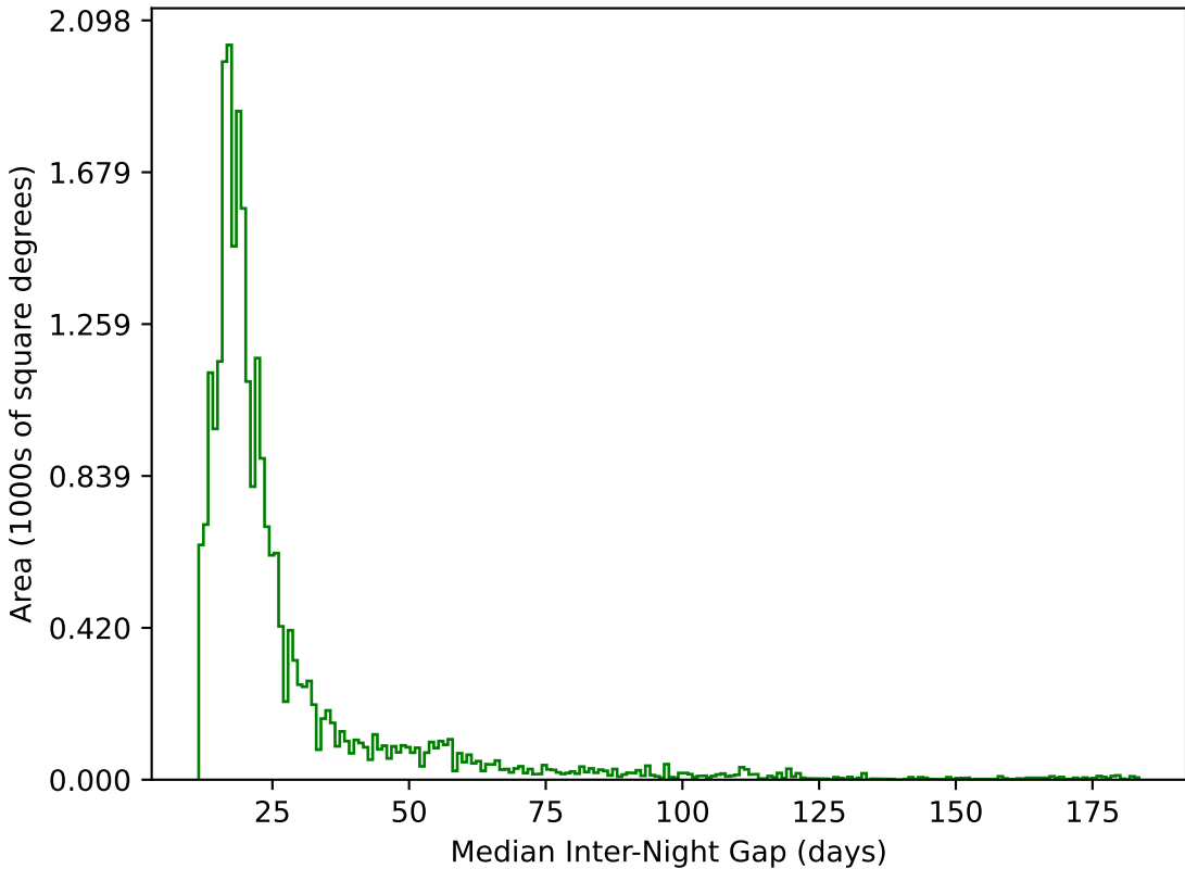
too_elab_r16_d2_giz_v3.4_10yrs All sky g band: Median Inter-Night Gap
