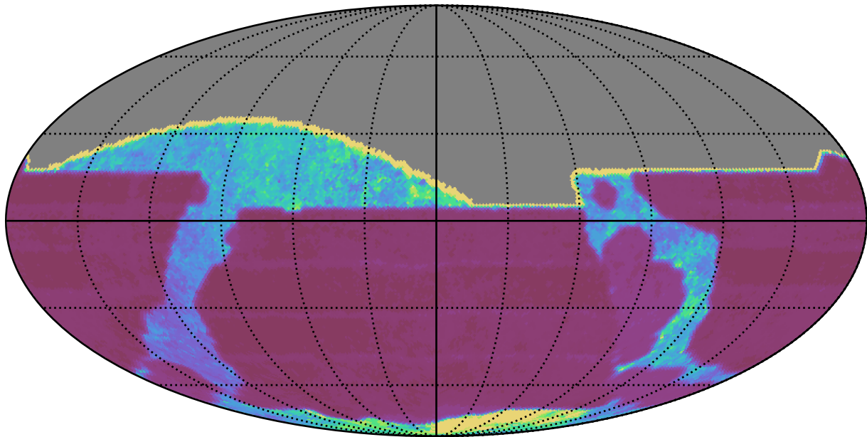
too_elab_r16_d2_giz_v3.4_10yrs All sky all bands: Median Inter-Night Gap
