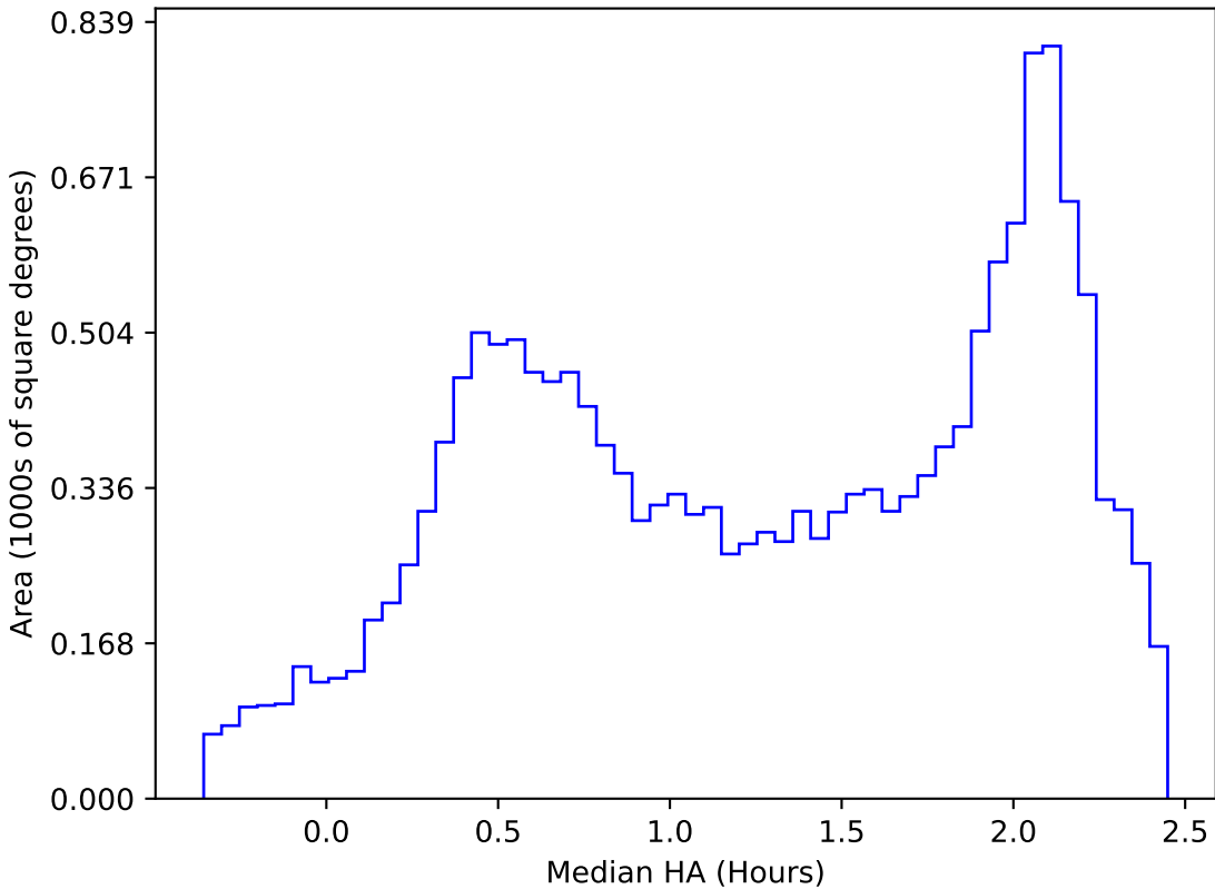
too_elab_r16_d2_giz_v3.4_10yrs WFD y band: Median HA
