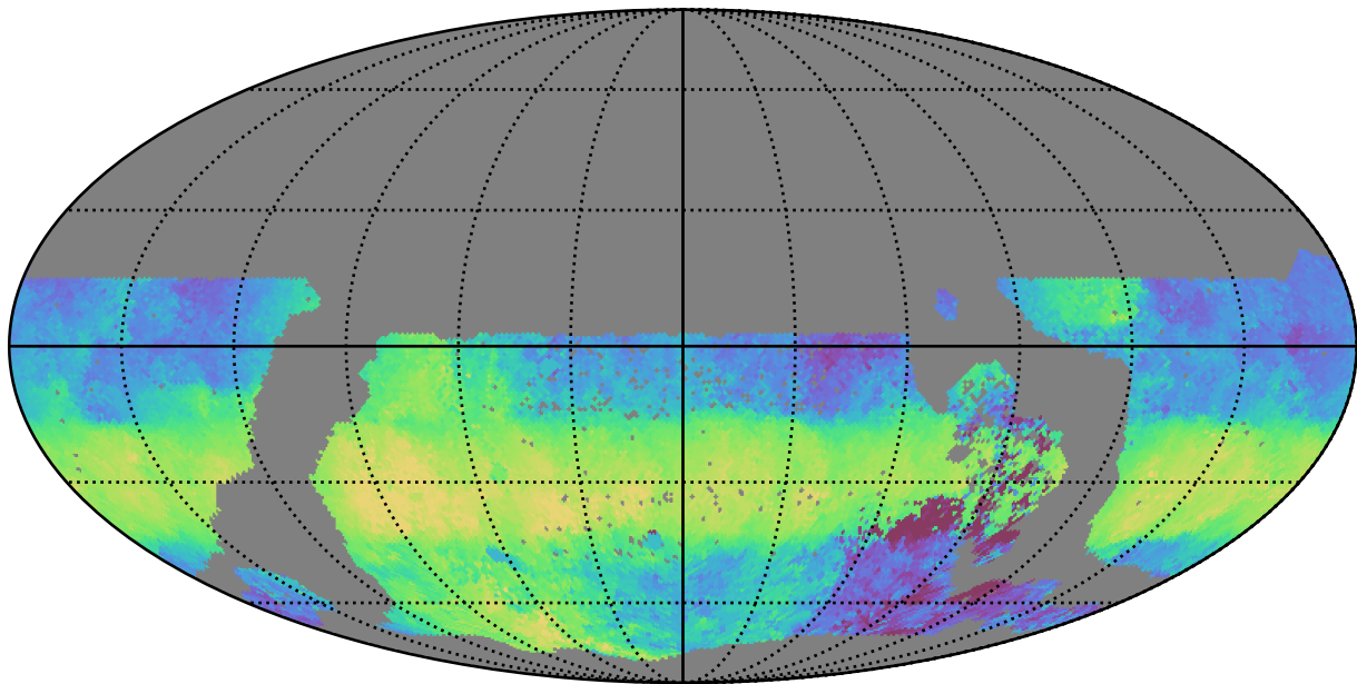
too_elab_r16_d2_giz_v3.4_10yrs WFD u band: Median HA
