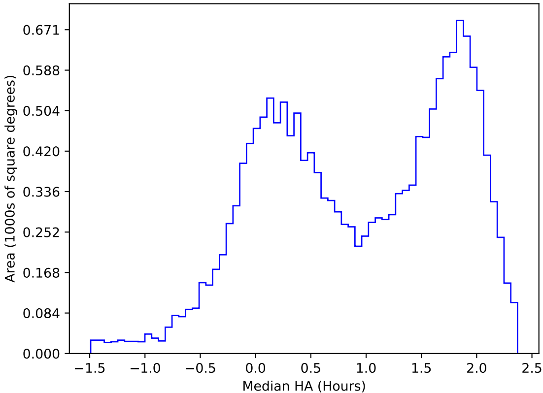
too_elab_r16_d2_giz_v3.4_10yrs WFD u band: Median HA
