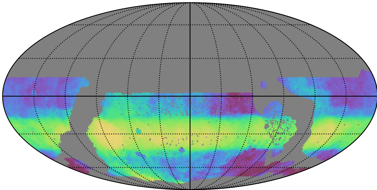
too_elab_r16_d2_giz_v3.4_10yrs WFD r band: Median HA
