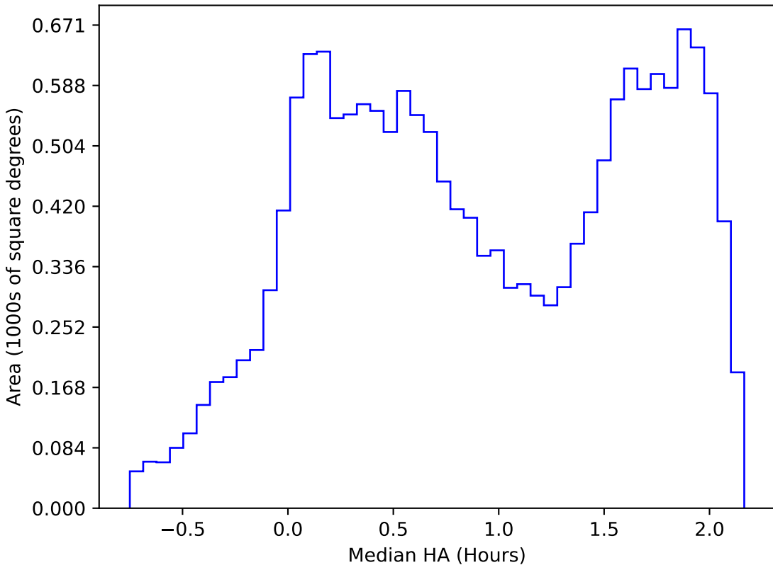
too_elab_r16_d2_giz_v3.4_10yrs WFD r band: Median HA
