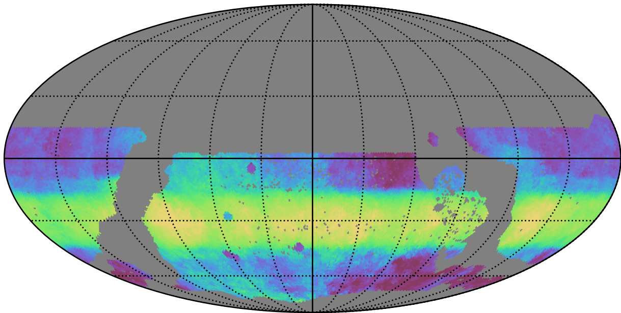
too_elab_r16_d2_giz_v3.4_10yrs WFD i band: Median HA
