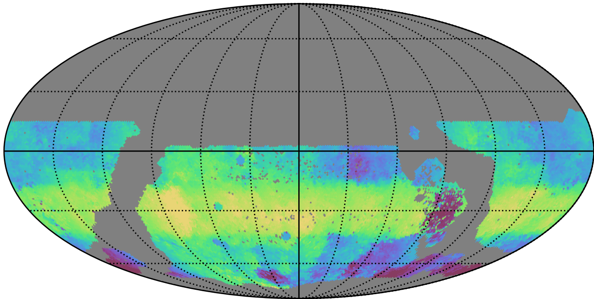
too_elab_r16_d2_giz_v3.4_10yrs WFD g band: Median HA
