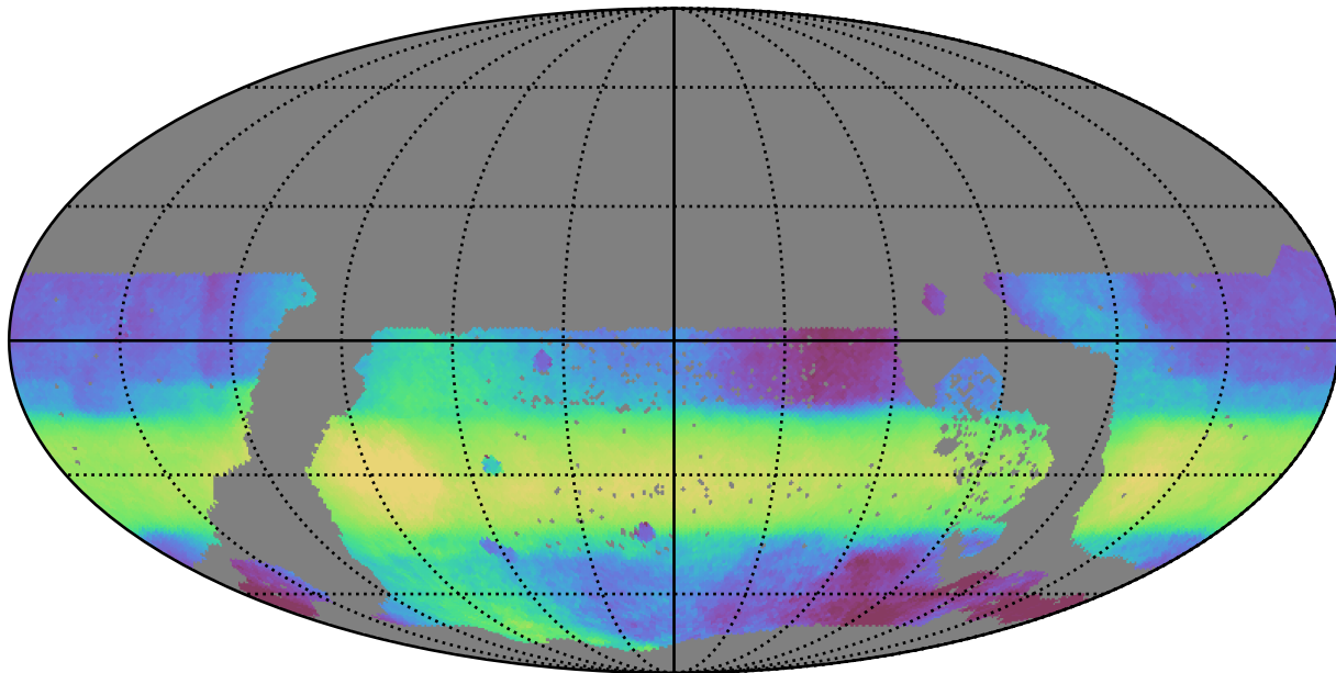
too_elab_r16_d2_giz_v3.4_10yrs WFD all bands: Median HA
