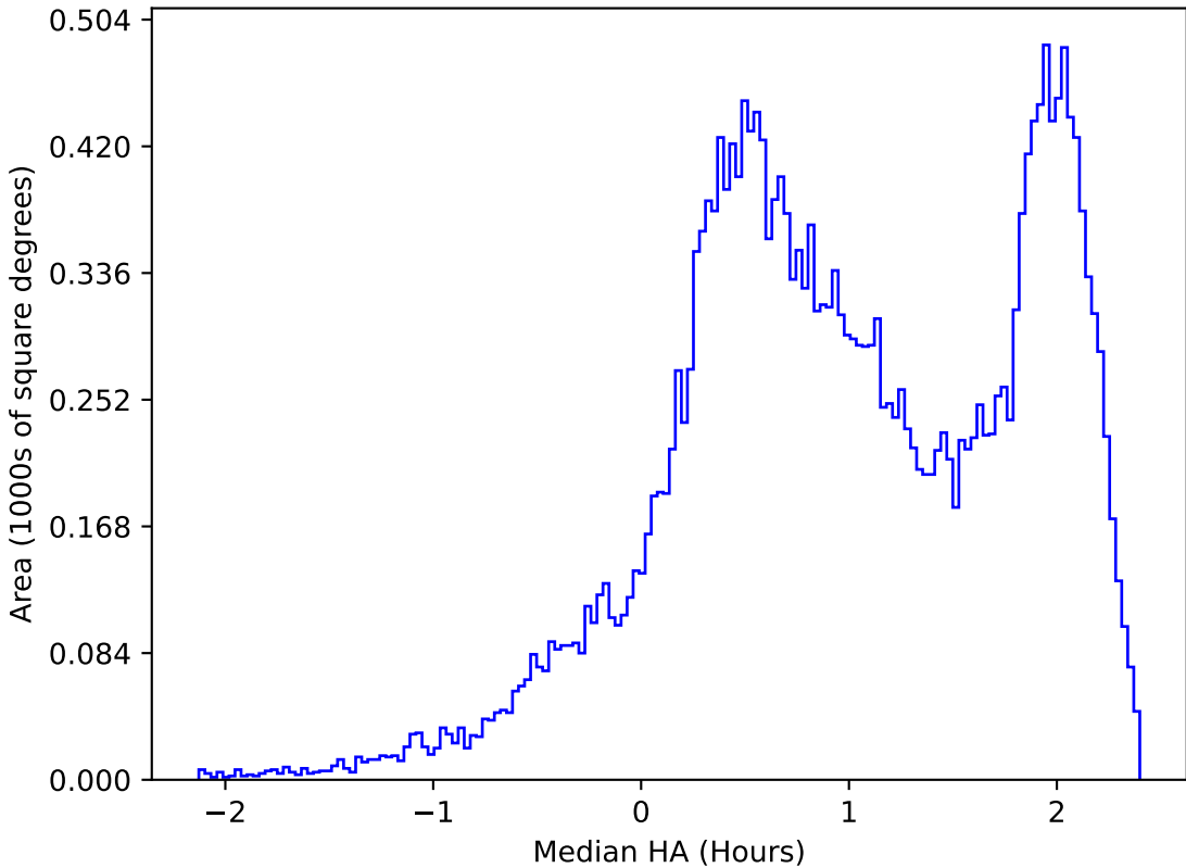
too_elab_r16_d2_giz_v3.4_10yrs All sky z band: Median HA
