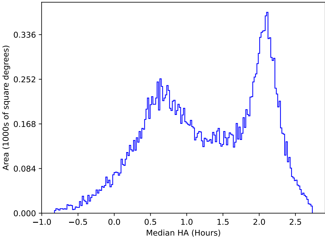
too_elab_r16_d2_giz_v3.4_10yrs All sky y band: Median HA
