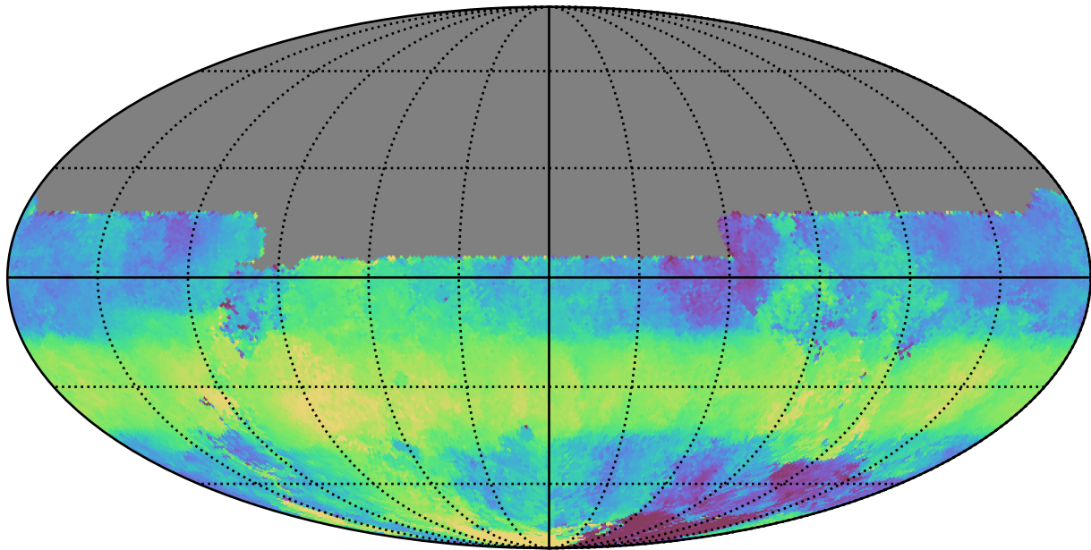
too_elab_r16_d2_giz_v3.4_10yrs All sky u band: Median HA
