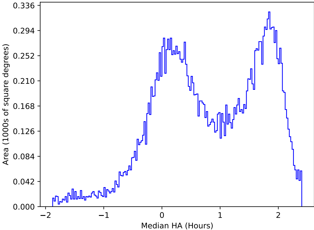
too_elab_r16_d2_giz_v3.4_10yrs All sky u band: Median HA
