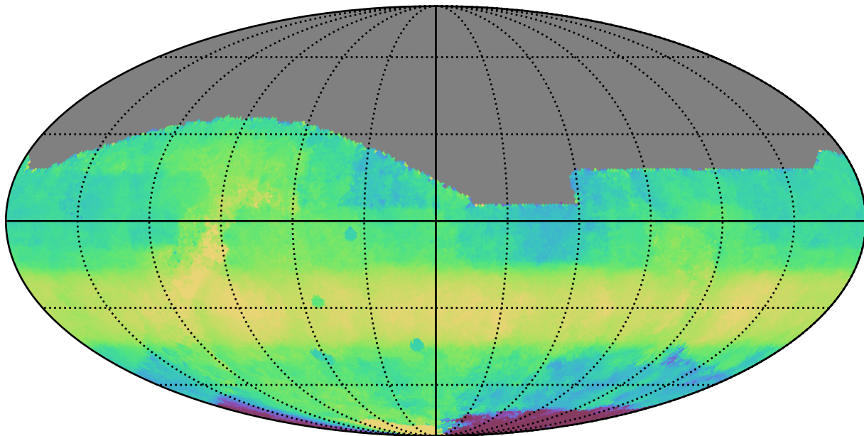
too_elab_r16_d2_giz_v3.4_10yrs All sky i band: Median HA
