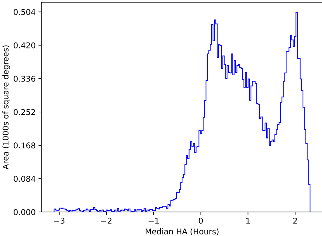
too_elab_r16_d2_giz_v3.4_10yrs All sky i band: Median HA
