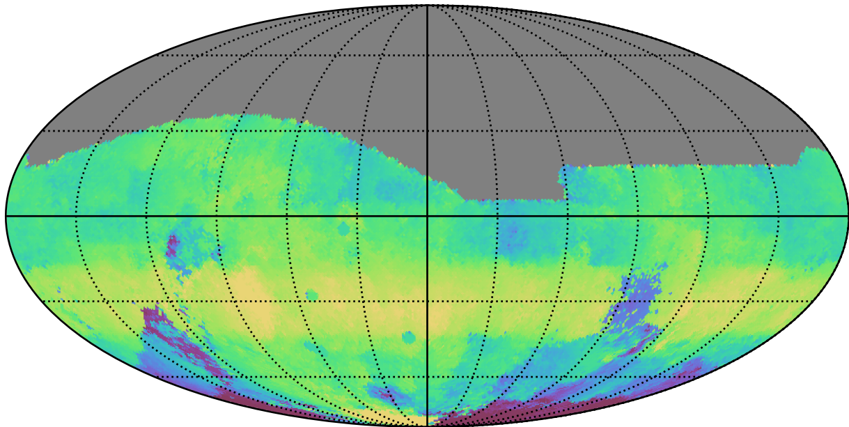
too_elab_r16_d2_giz_v3.4_10yrs All sky g band: Median HA
