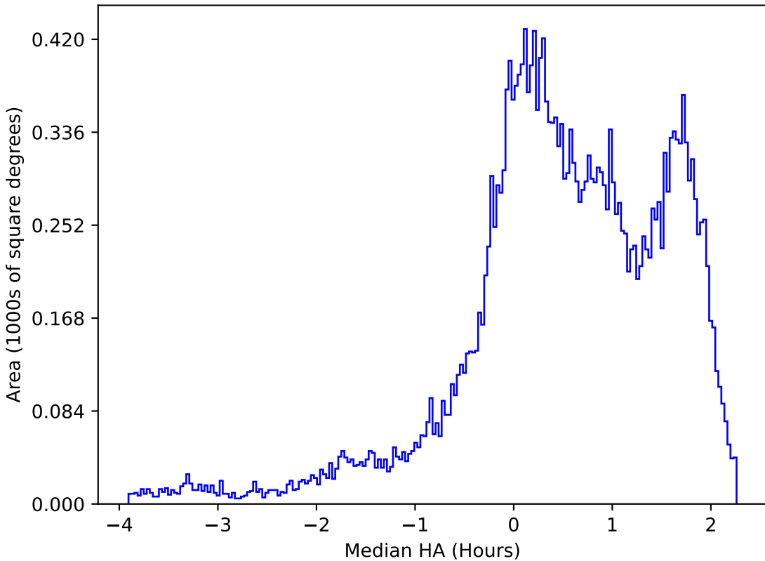
too_elab_r16_d2_giz_v3.4_10yrs All sky g band: Median HA
