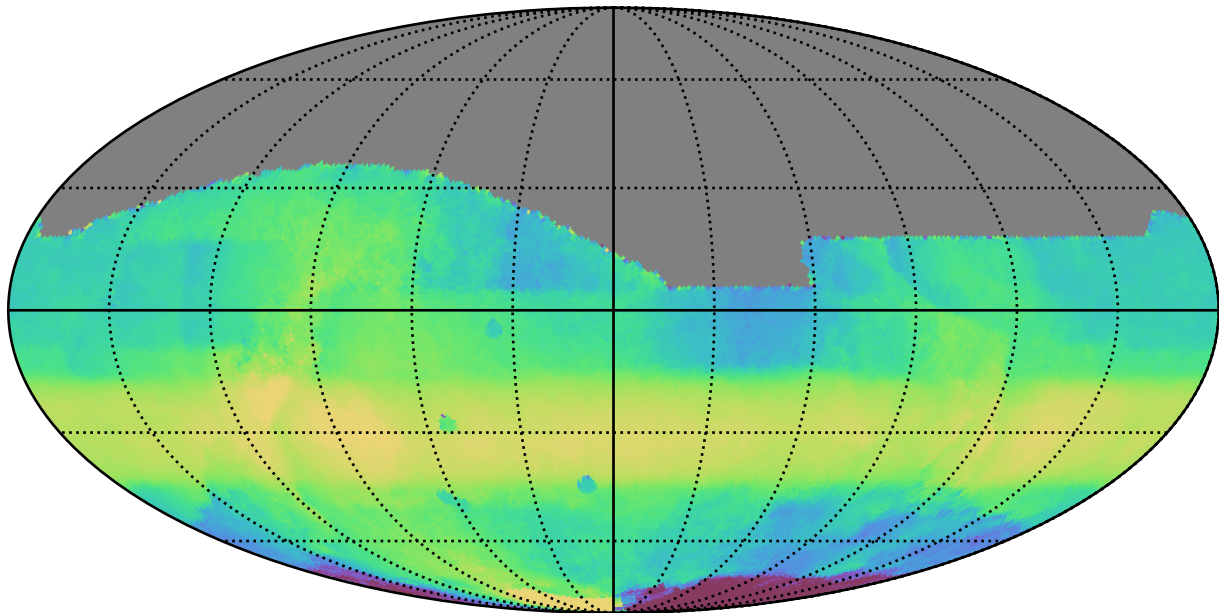
too_elab_r16_d2_giz_v3.4_10yrs All sky all bands: Median HA
