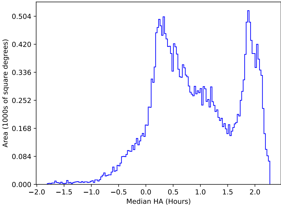
too_elab_r16_d2_giz_v3.4_10yrs All sky all bands: Median HA
