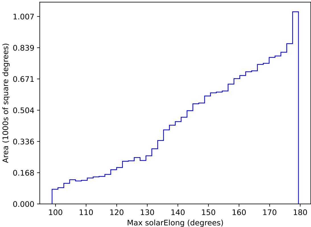
too_elab_r16_d2_giz_v3.4_10yrs WFD z band: Max solarElong
