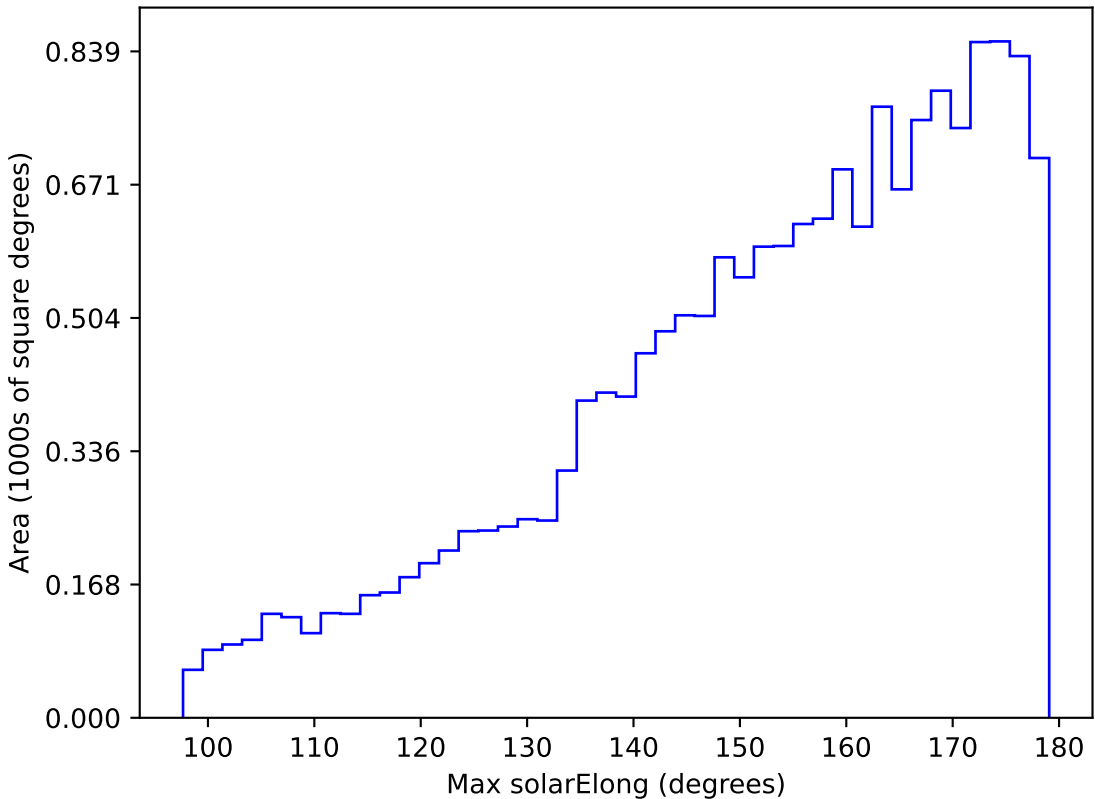
too_elab_r16_d2_giz_v3.4_10yrs WFD u band: Max solarElong
