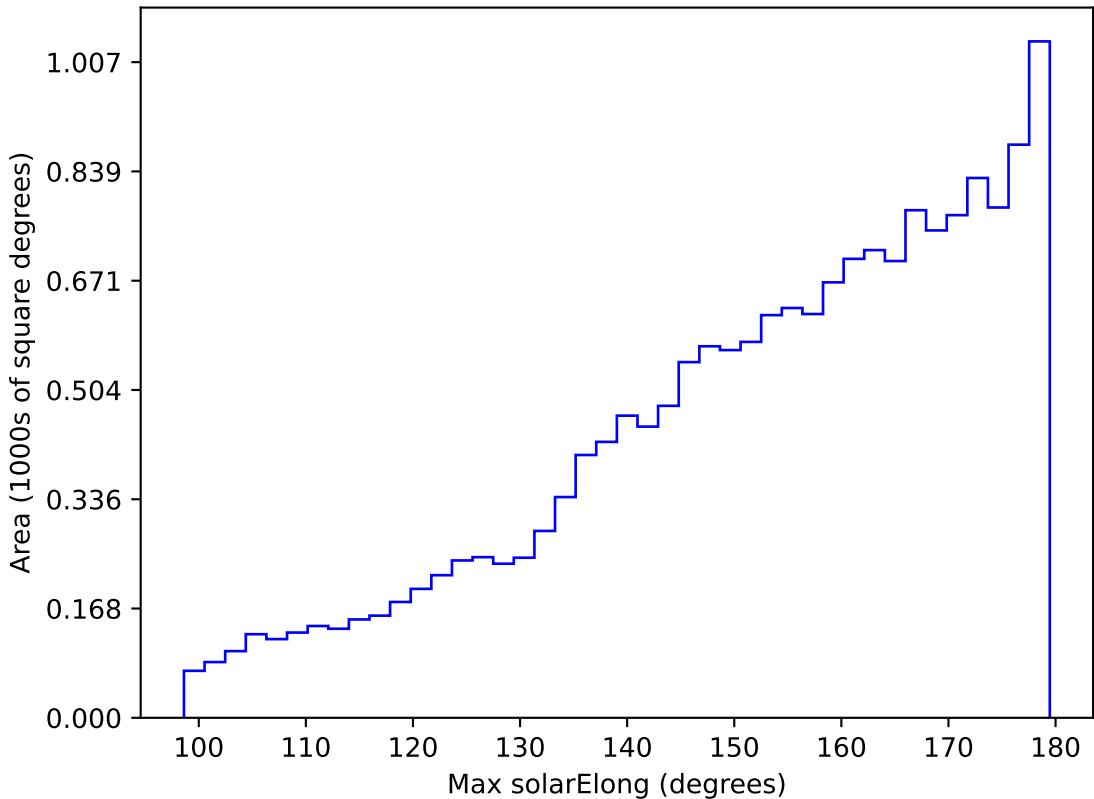
too_elab_r16_d2_giz_v3.4_10yrs WFD r band: Max solarElong
