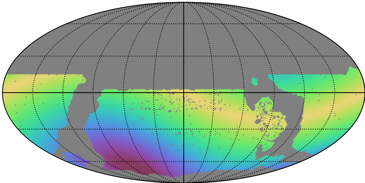
too_elab_r16_d2_giz_v3.4_10yrs WFD i band: Max solarElong
