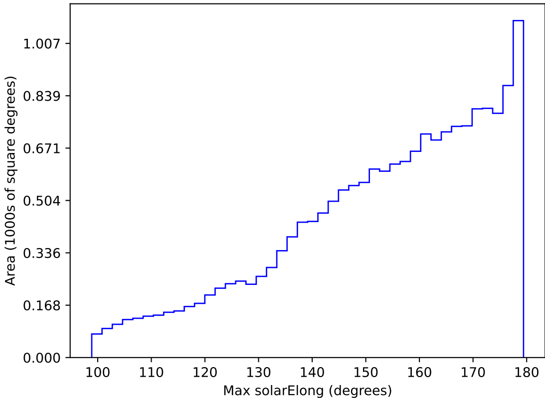
too_elab_r16_d2_giz_v3.4_10yrs WFD i band: Max solarElong
