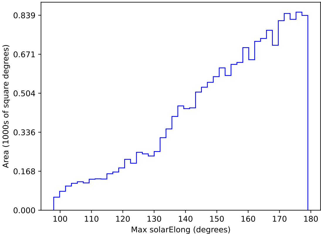
too_elab_r16_d2_giz_v3.4_10yrs WFD g band: Max solarElong
