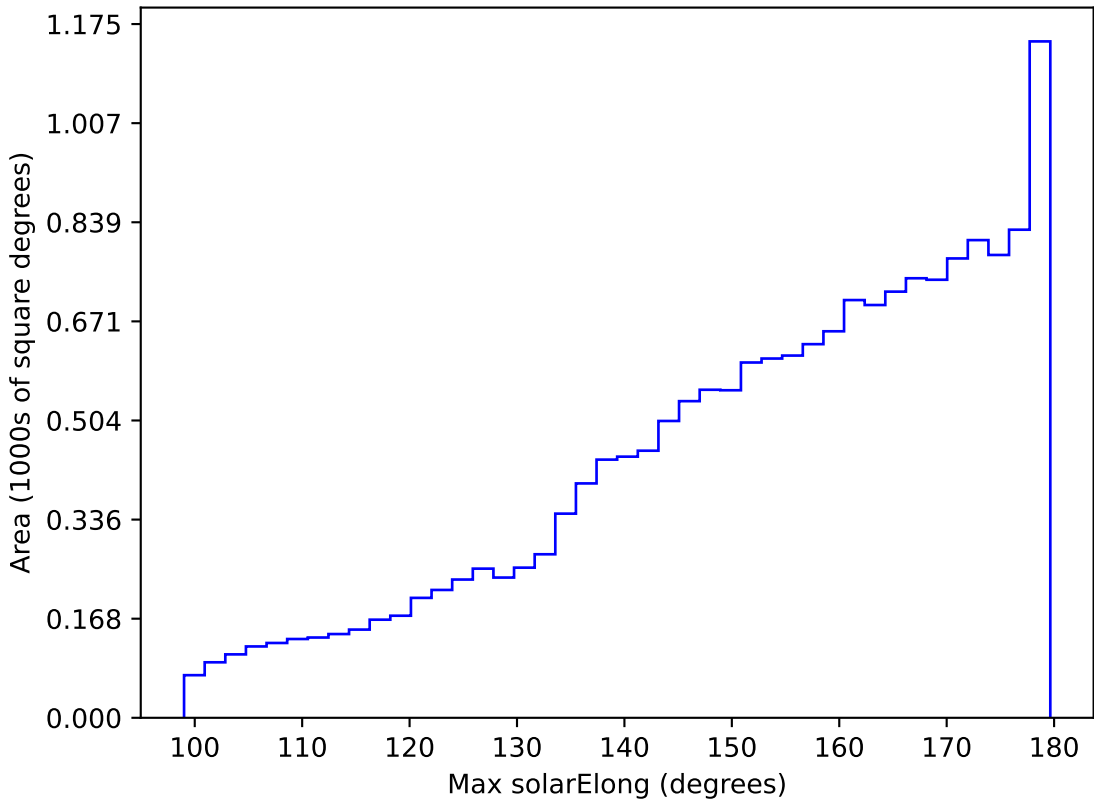
too_elab_r16_d2_giz_v3.4_10yrs WFD all bands: Max solarElong
