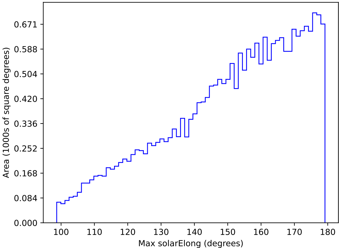
too_elab_r16_d2_giz_v3.4_10yrs All sky y band: Max solarElong
