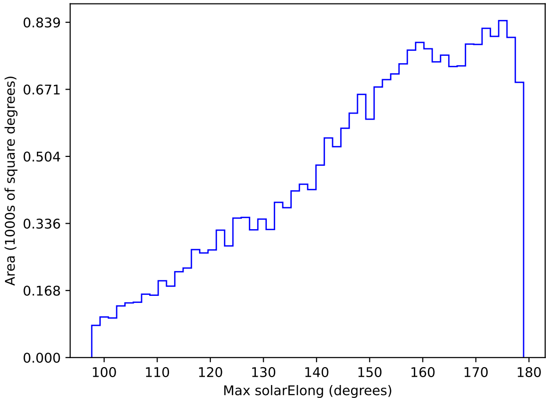
too_elab_r16_d2_giz_v3.4_10yrs All sky u band: Max solarElong
