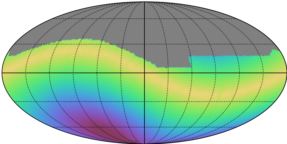
too_elab_r16_d2_giz_v3.4_10yrs All sky r band: Max solarElong
