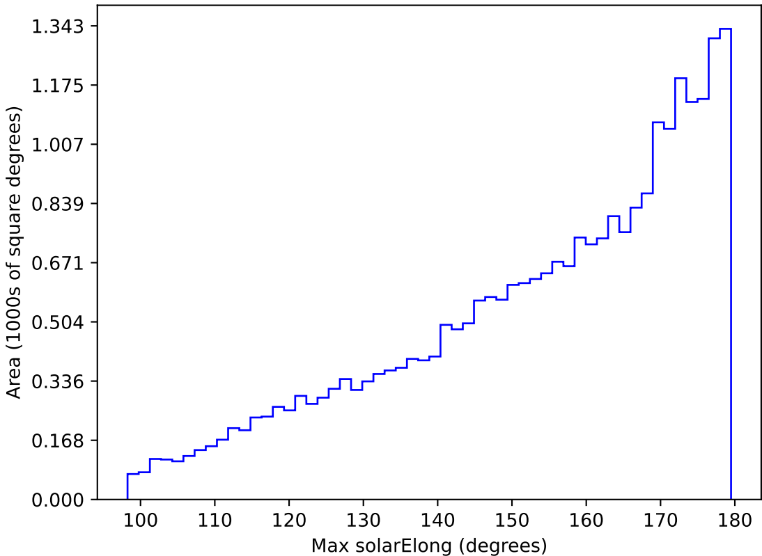
too_elab_r16_d2_giz_v3.4_10yrs All sky r band: Max solarElong
