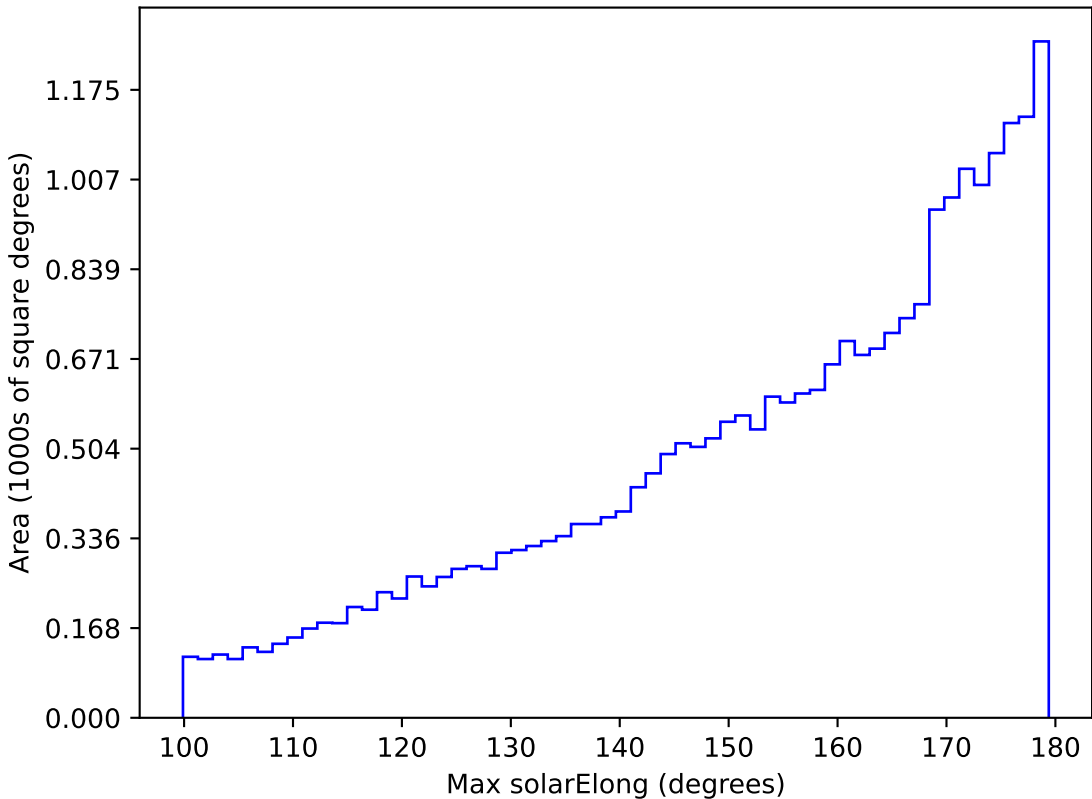
too_elab_r16_d2_giz_v3.4_10yrs All sky i band: Max solarElong
