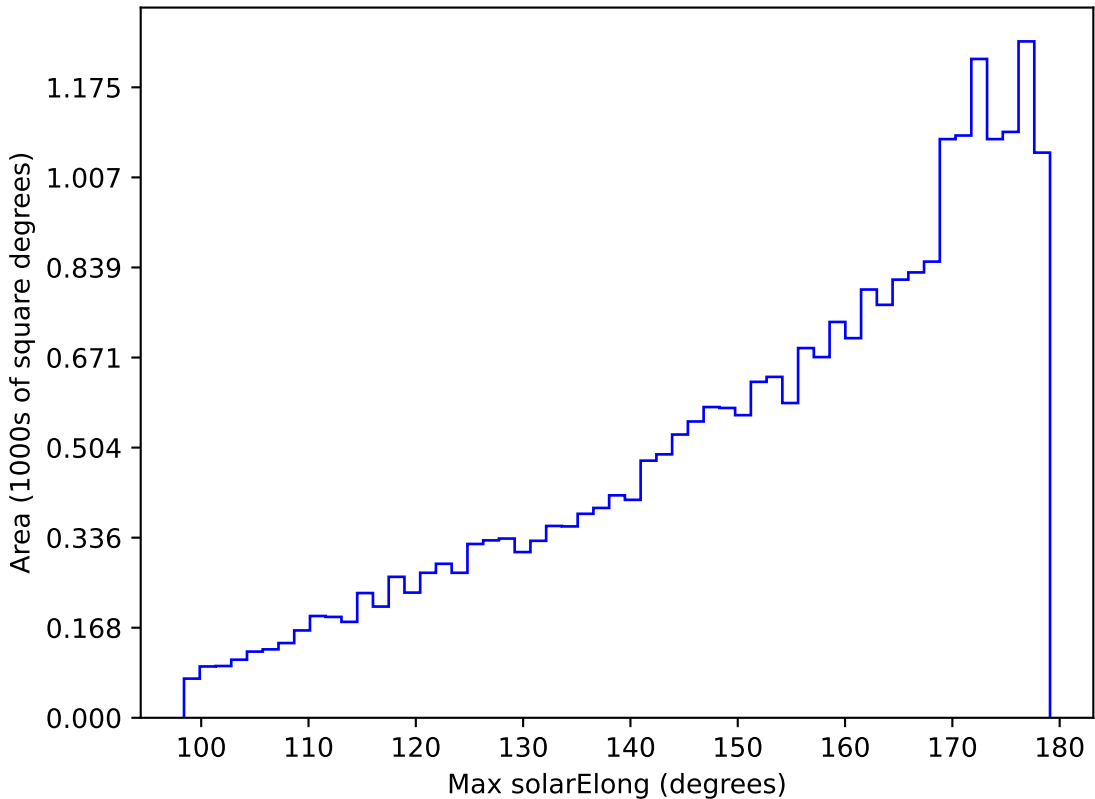
too_elab_r16_d2_giz_v3.4_10yrs All sky g band: Max solarElong
