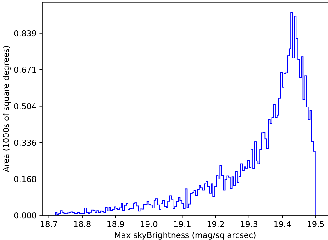
too_elab_r16_d2_giz_v3.4_10yrs Yr 1 z band: Max skyBrightness
