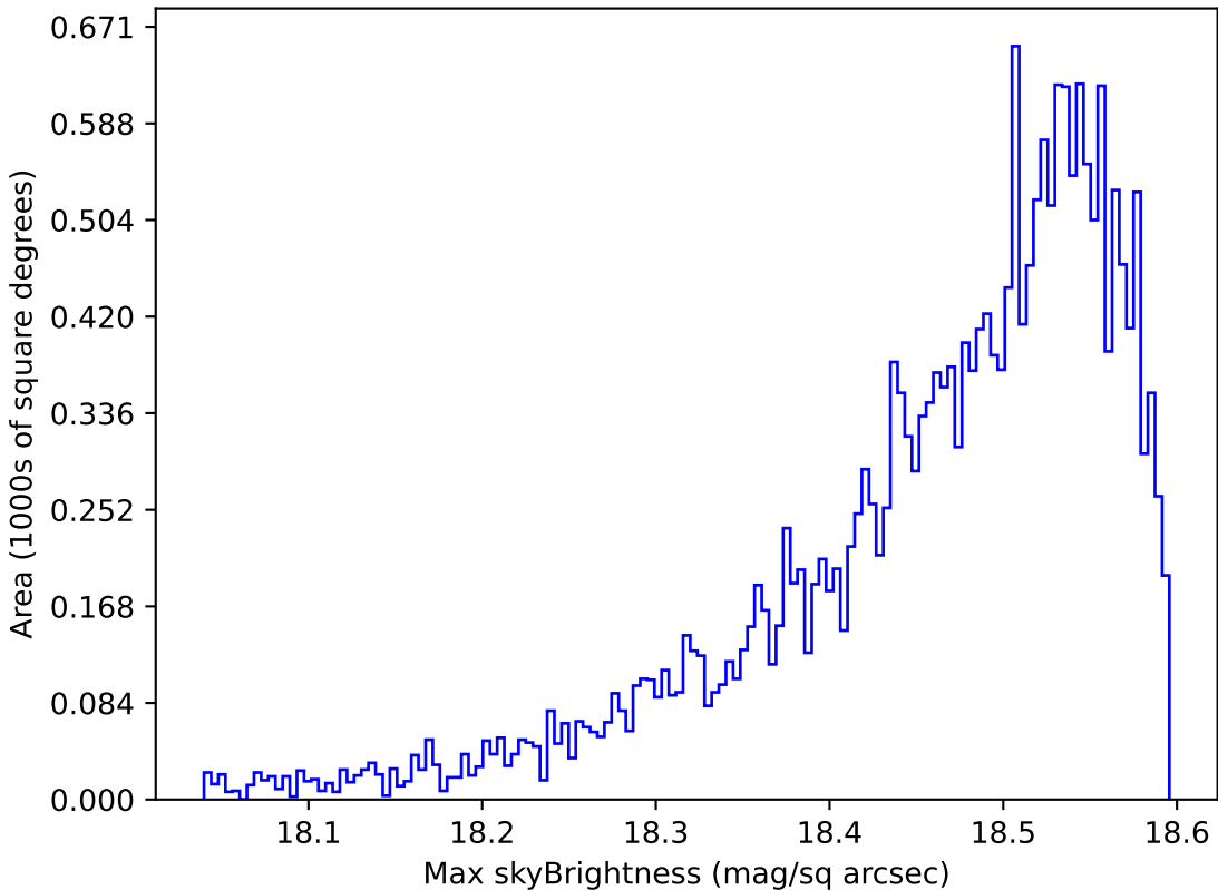
too_elab_r16_d2_giz_v3.4_10yrs Yr 1 y band: Max skyBrightness
