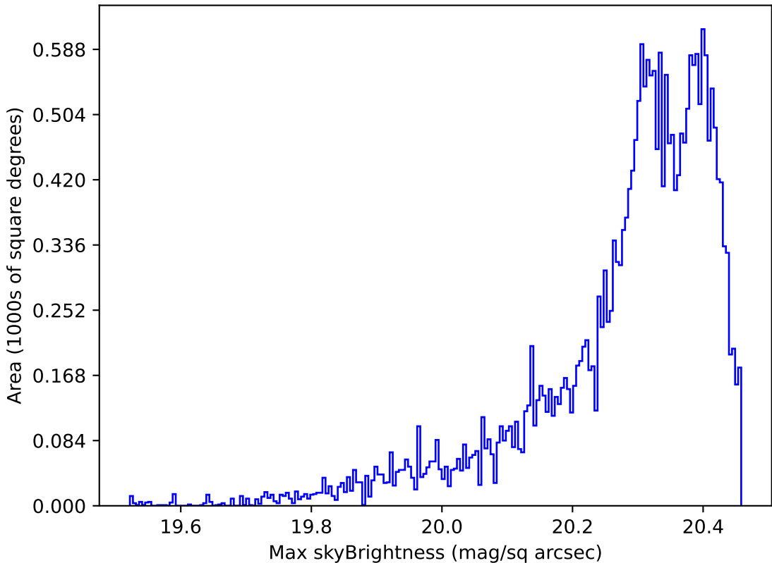
too_elab_r16_d2_giz_v3.4_10yrs Yr 1 i band: Max skyBrightness
